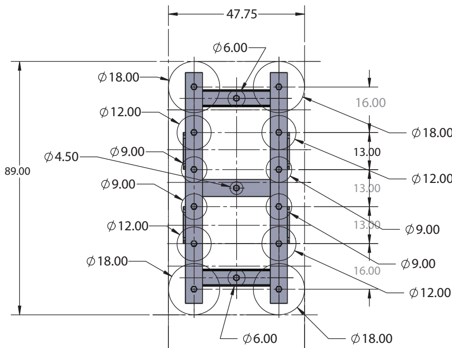
SHOWN WITH AN ASSORTMENT OF VARIOUS SIZE AUGERS. AUGER SIZES CAN VARY WITHIN SIZE LIMITATIONS OF PALLET
